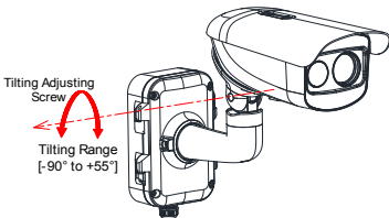
Figure 2-24 T-Axis Adjustment
