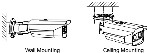
Figure 2-15 Wall/Ceiling Mounting
