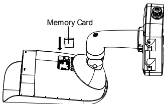
Figure 2-8 Insert Memory Card
