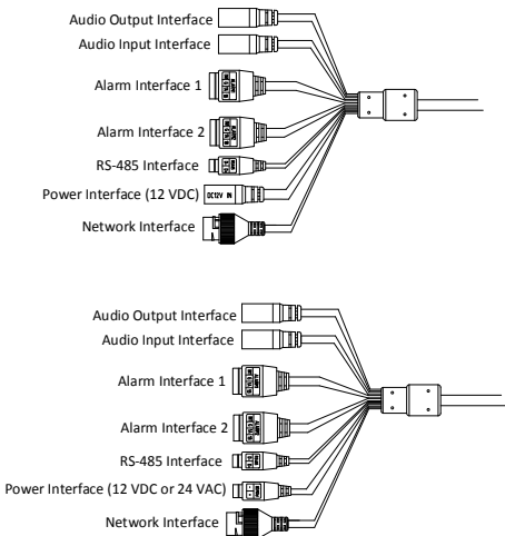
Figure 1-8 Cable Description
