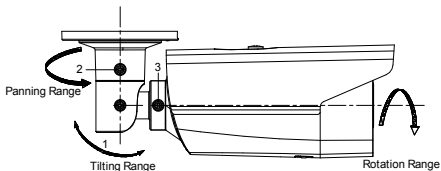
Figure 2-16 3-Axis Adjustment
