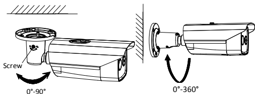
Figure 2-17 2-Axis Adjustment
