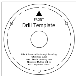
Figure 2-14 Drill Template
