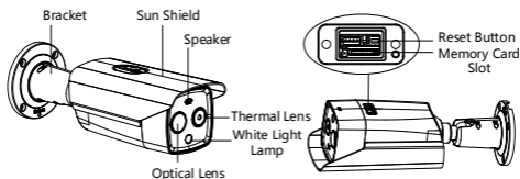
Figure 1-7 Type IV Camera Appearance
