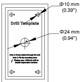
Figure 2-20 Drill Template
