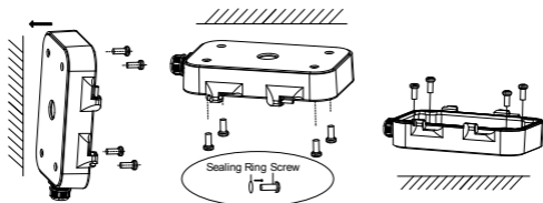
Figure 2-21 Install Junction Box Base
