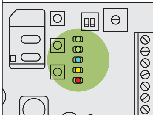
Fig. 17: LED-indikatorer
